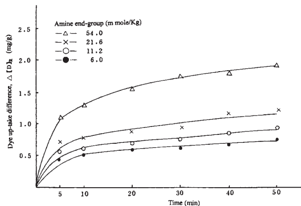
Figure 15 Relationship of dye uptake difference and reaction time with various amino end groups and pH = 3.
