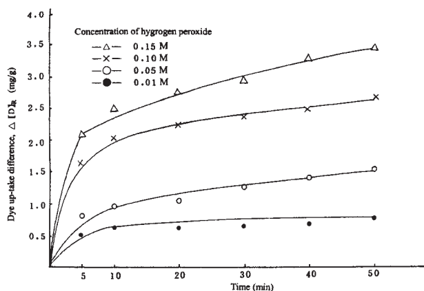
Figure 13 Relationship of dye uptake difference and reaction time at various concentrations of hydrogen peroxide and pH = 3.
